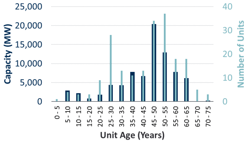
Figure 3: Coal Fleet Characterization
