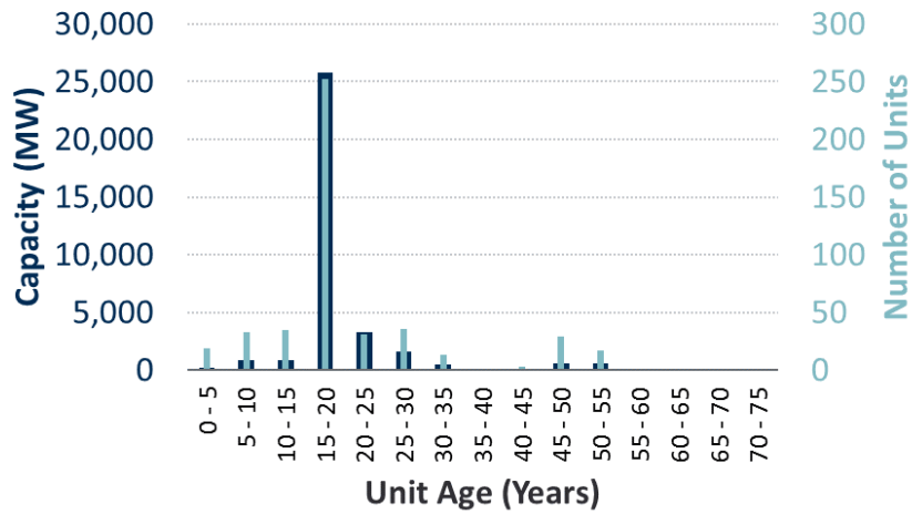
Figure 5: Natural Gas Combustion Turbine Fleet Characterization
