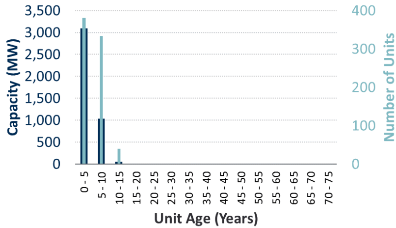
Figure 7: Large-Scale Solar Photovoltaic Fleet Characterization
