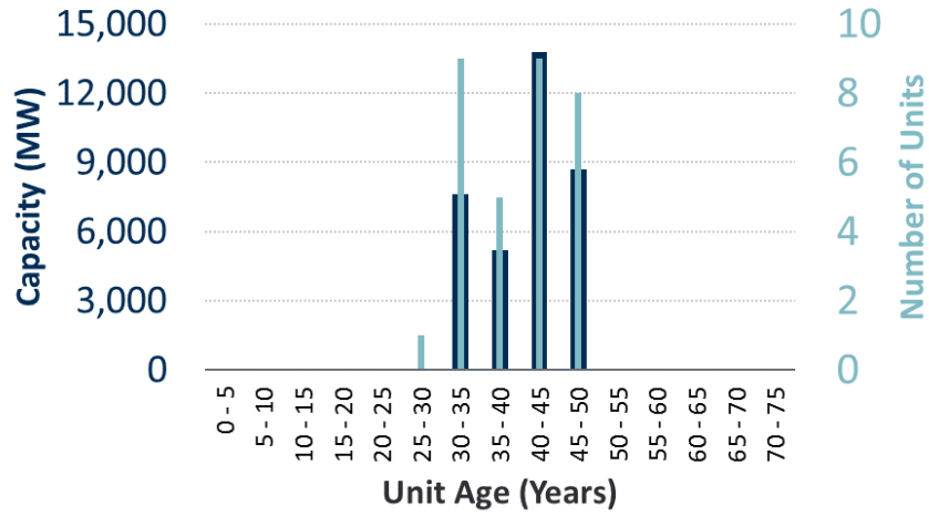
Figure 2: Multi-Unit Nuclear Fleet Characterization
