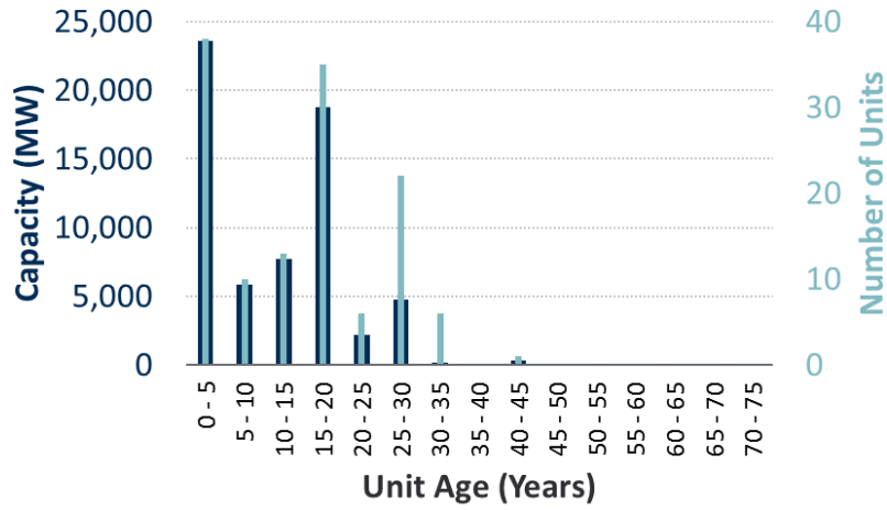
Figure 4: Natural Gas Combined-Cycle Fleet Characterization
