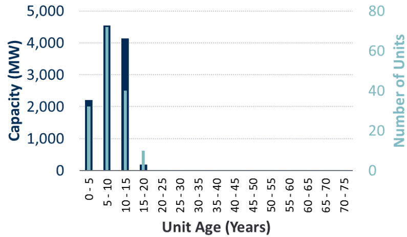
Figure 6: Onshore Wind Fleet Characterization
