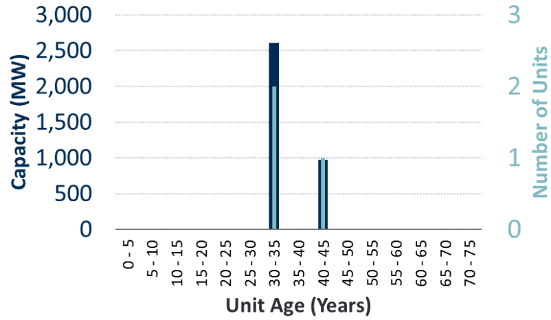
Figure 1: Single-Unit Nuclear Fleet Characterization
